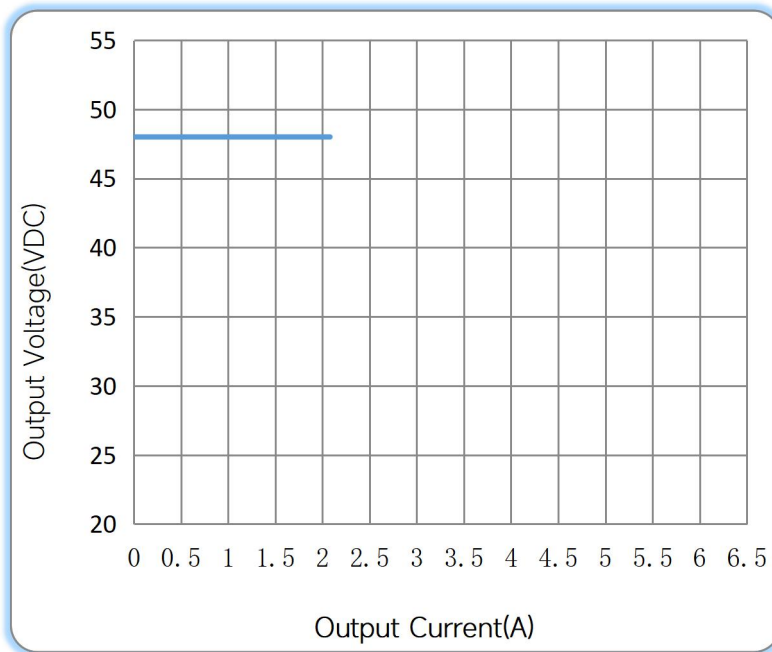
— Operating window 100%
