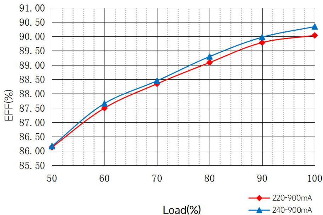
Efficiency vs. Load
