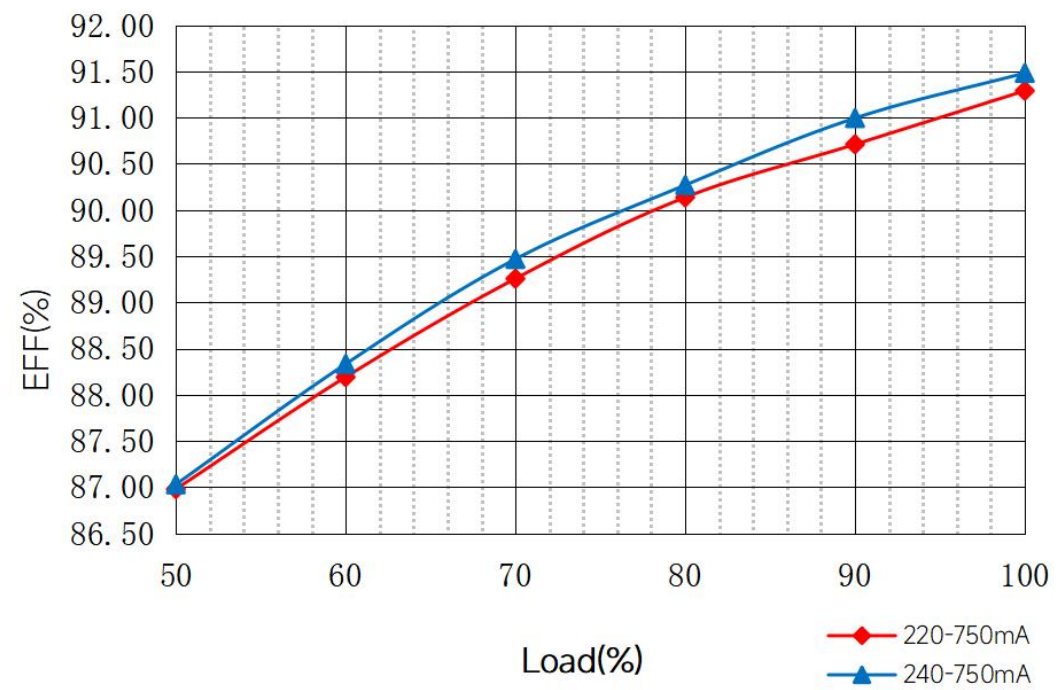
Efficiency vs. Load
