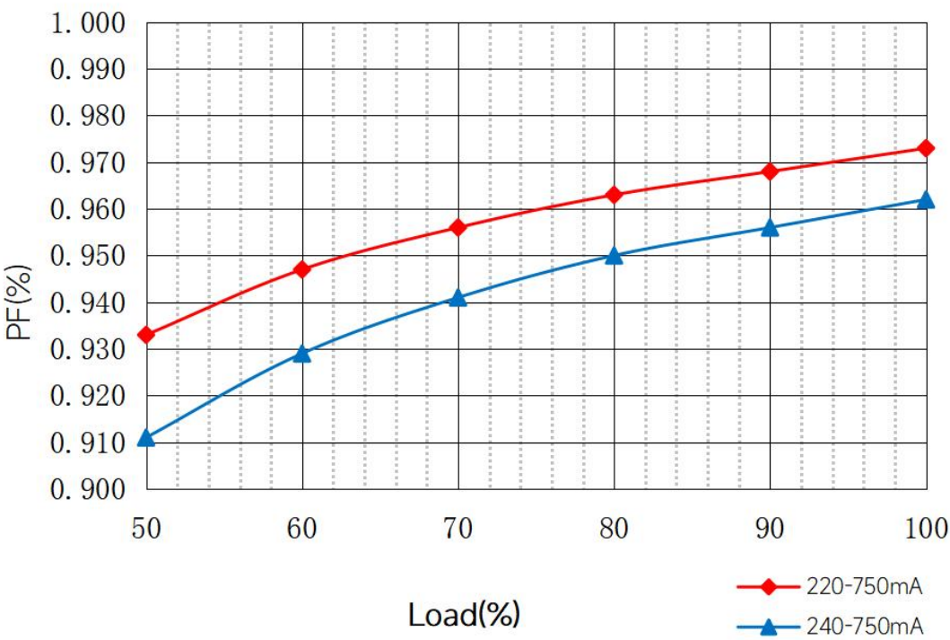
Power Factor Characteristics
