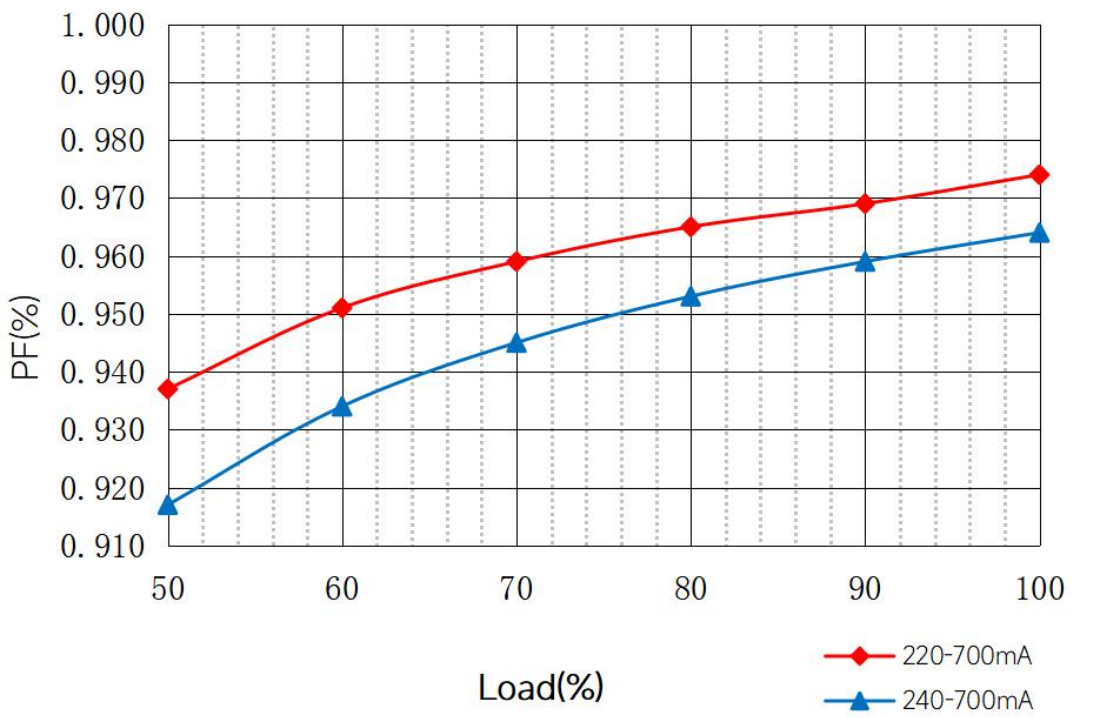
Power Factor Characteristics
