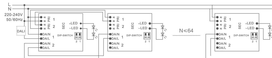
Image5 DALI wiring
