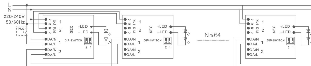
Image4 Push wiring
